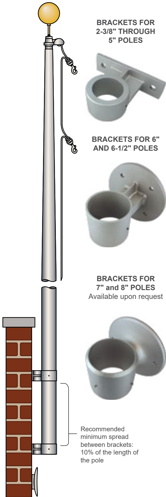
Illustration depicting 5-6" butt dia. poles
