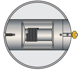
M-Winch Detail
