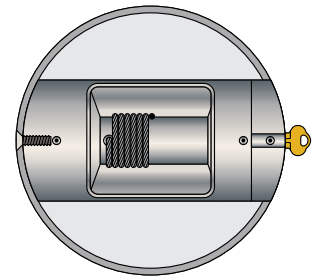
M-Winch Detail
